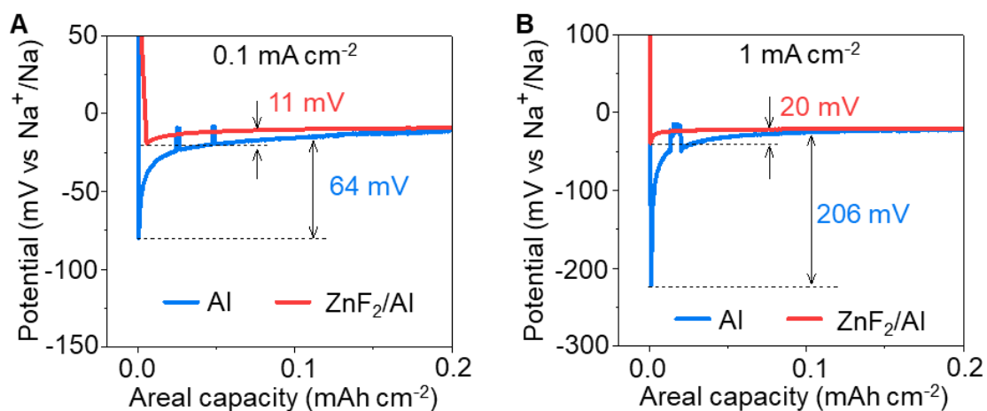
Figure S10. Overpotential of Na nucleation on bare Al and \text{ZnF}_2/\text{Al} . A) At a current density of 0.1 \text{ mA cm}^{-2} . B) At a current density of 1.0 \text{ mA cm}^{-2} .
