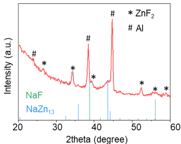
Figure S9. XRD pattern of the sodiated \text{ZnF}_2/\text{Al} with 2500 ALD cycles. To improve the detectability of the Na–Zn alloy phase, a thicker \text{ZnF}_2 coating was deposited on Al by increasing the ALD cycle number to 2500 cycles (corresponding to \sim 220 nm). The resulting \text{ZnF}_2/\text{Al} -2500 electrode subsequently underwent the sodiation process under the same conditions used for the 625-cycle sample.
